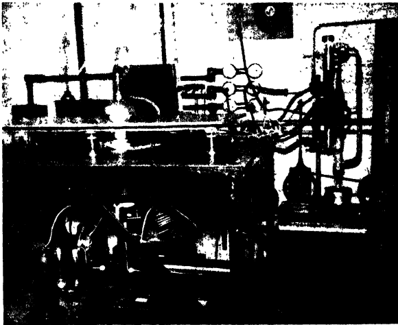
FIG. 7.—Photograph of Hadding-Siegbahn-type tube set-up. (Courtesy of New Jersey Zinc Company.)
